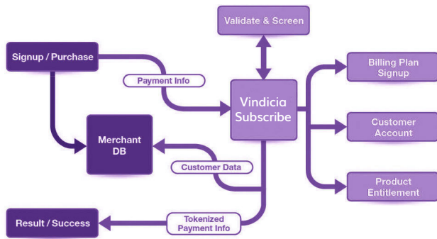
Figure 2: Transaction flow with HOA capabilities
